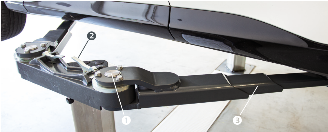
Swing arm support with tool tray.
