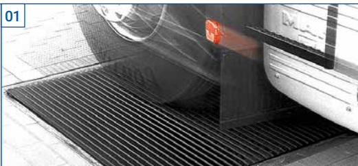
The side-slip tester MINC II EURO ensures that the axle geometry is inspected within seconds once the test vehicle passes over it (up to 15.0 t axle load) as well as a fully automatic evaluation of the deviation in m/km.
